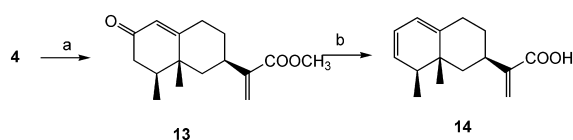
Scheme 3. Reagents and conditions: (a) \text{MeOH}/\text{HCl} , reflux (92%); (b) \text{AlCl}_3 , \text{LiAlH}_4 , \text{THF} , 0 °C (82%).
