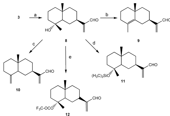
Scheme 2. Reagents and conditions: (a) Jones reagent (87%); (b) TsOH, C 6 H 6 , MS 4 Å, 80 °C (93%); (c) POCl 3 , pyridine, –20 °C (56%); (d) HMDS, TMSCl, CH 2 Cl 2 , rt (91%); (e) (F 3 CCO) 2 O, pyridine, DMAP, rt (92%).
