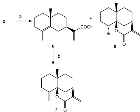
Scheme 1. Reagents and conditions: (a) TsOH, C 6 H 6 , MS 4 Å, 80 °C (after silica gel chromatography 55% 5 and 46% 6 ); (b) (i) i -Pro, bengal rose, sunlight, 48 h, (ii) MeOH, triphenylphosphine, rt, overnight; (iii) Ac 2 O, pyridine, rt, overnight (72%).
